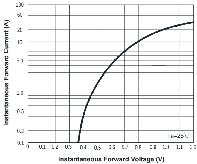
FIG3: Forward Voltage
