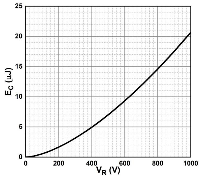
Figure 6. Capacitance Stored Energy
