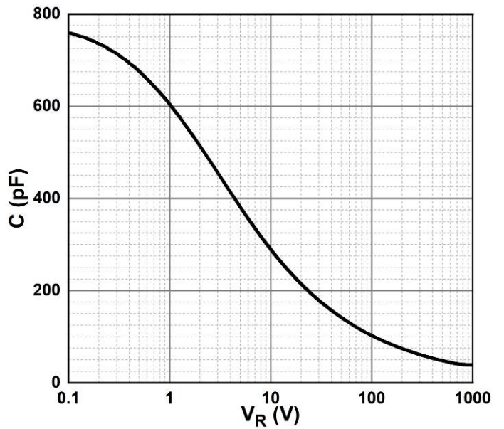
Figure 4. Capacitance vs. Reverse Voltage
