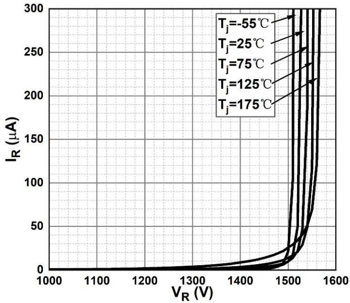
Figure 3. Reverse Characteristics
