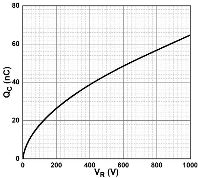
Figure 5. Total Capacitance Charge vs. Reverse Voltage
