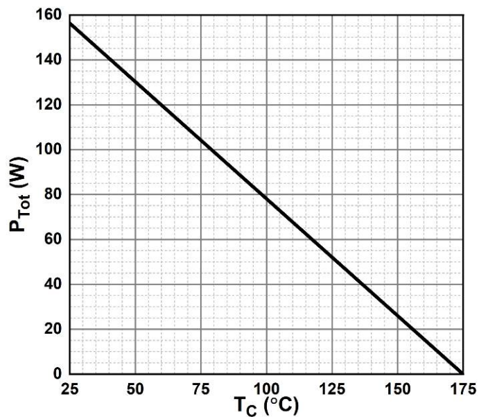
Figure 7. Power Derating
