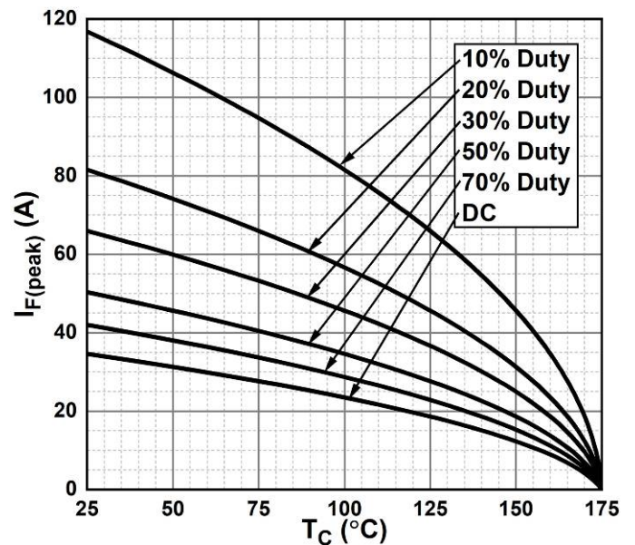
Figure 8. Current Derating
