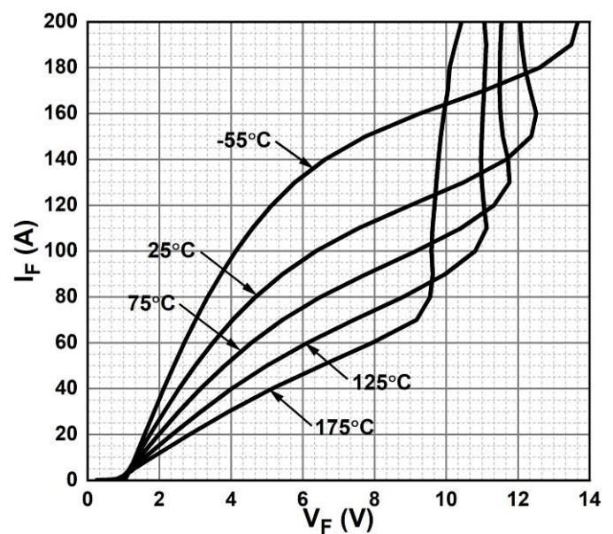
Figure 2. Forward Characteristics in Surge Current
