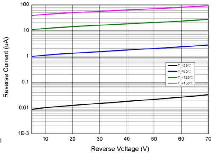
Fig.4: Reverse Characteristics
