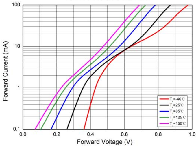
Fig.3: Forward Characteristics
