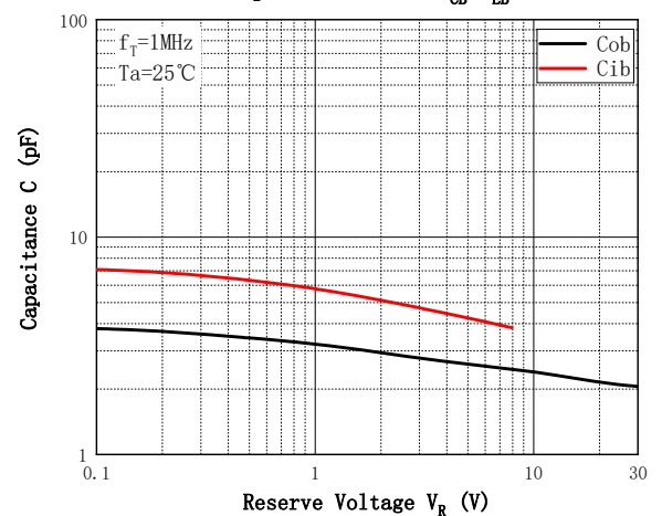
Fig.6 - C_{ob}/C_{ib}-V_{CE}/V_{EB}
