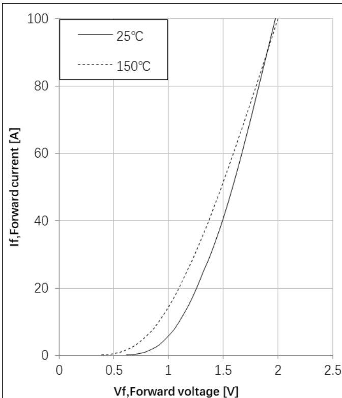
Fig17. Diode forward current as a function of forward voltage
